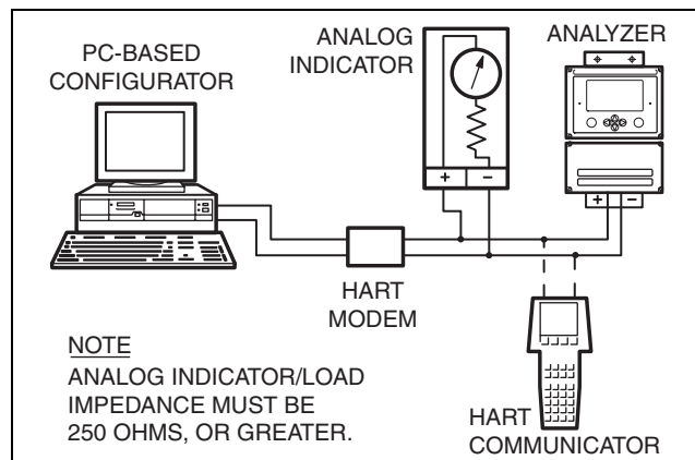
Figure 8. Point-to-Point Communications 4 to 20 mA Output with HART
