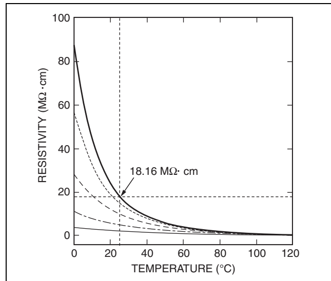
Figure 6. Temperature/Resistivity Relationship
