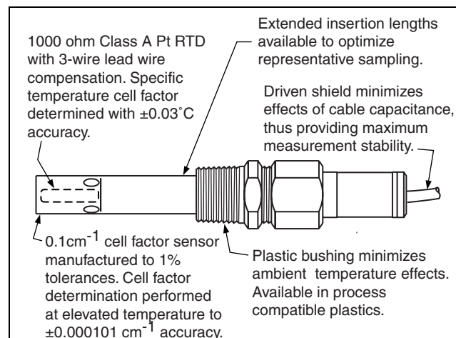
Figure 5. 871CR-B Sensor
