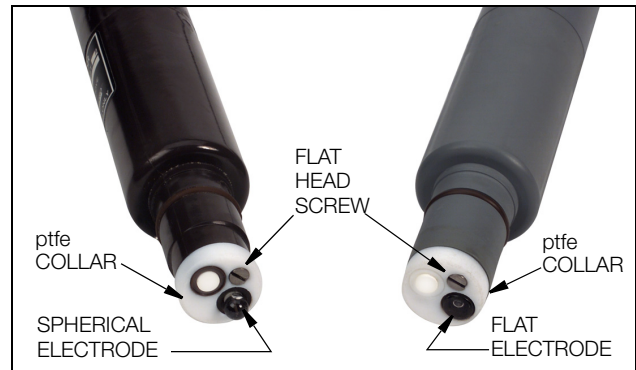
Figure 1. ptfe Collar (Option -T) Shown with Spherical Electrode (left) and Flat Glass Electrode (right)
