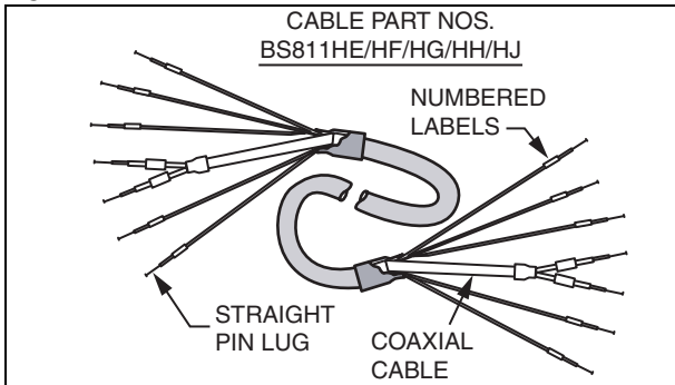
Figure 13. Extension Cable Assemblies when No Preamplifier is used
