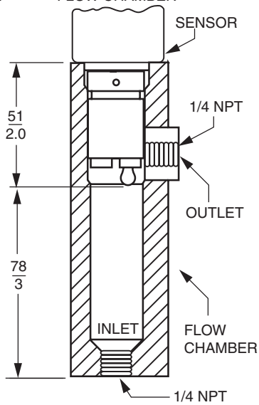
PVC FOXBORO PART 0051181 316 ss FOXBORO PART 0051179
