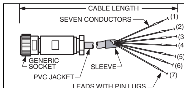
Figure 11. Patch Cord with Generic Connector Socket
