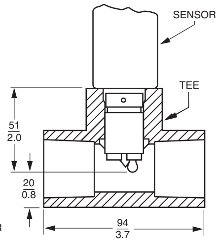
DN 25 OR 1 in (PVC) FOXBORO PART 0051184
