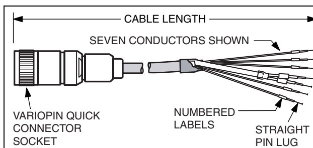
Figure 12. Patch Cord with Variopin Quick Connector Socket
