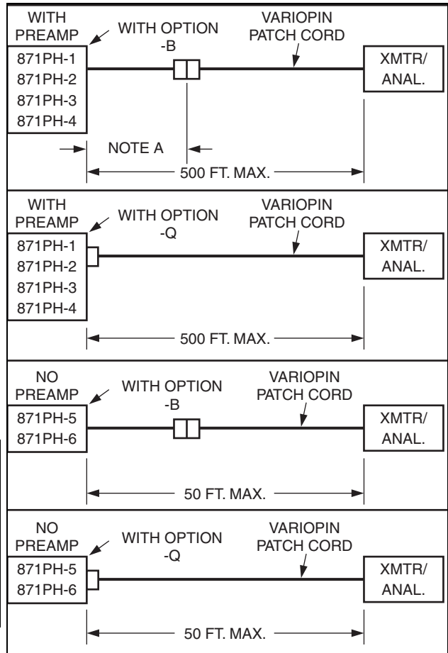
Figure 17. System Installation Topologies using Patch Cord with Variopin Quick Connector
