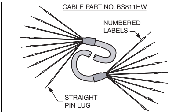
Figure 14. Extension Cable Assembly when a Preamplifier is used
