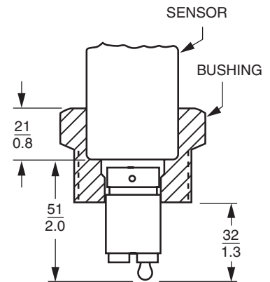
1 1/2 NPT (316 ss) FOXBORO PART 0051186
