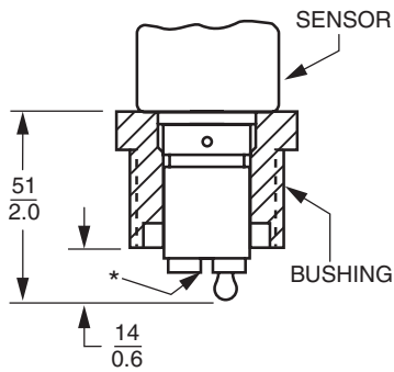
1 1/4 NPT (PVC) FOXBORO PART 0051183
