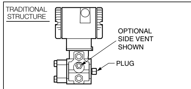
Figure 7. Vertical Mounting - Cavity Venting and Self-Draining into Process Line
