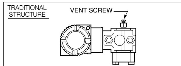
Figure 6. Horizontal Mounting - Cavity Venting and Self-Draining into Process Line
