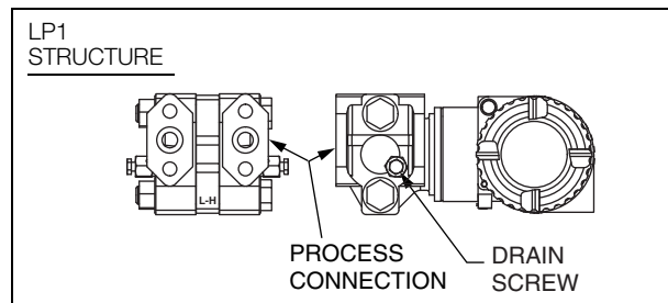
Figure 13. Horizontal Mounting with Drain Screw
