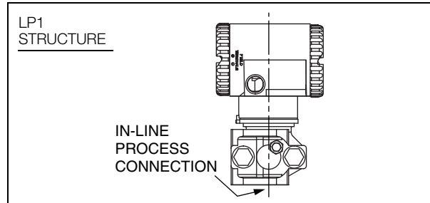
Figure 8. Low Profile Structure - LP1 Shown
