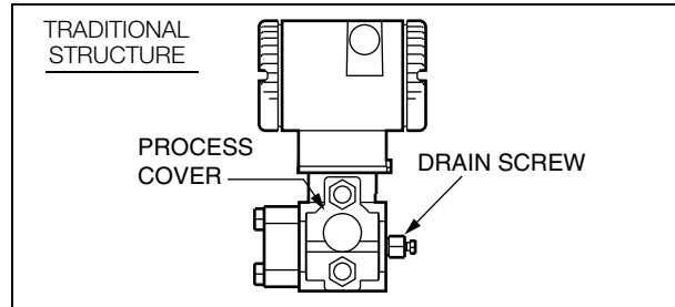
Figure 5. Vertical Mounting - Cavity Draining
