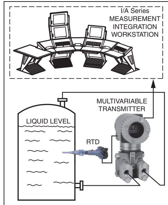
Figure 1. Typical Application for Liquid Level Measurement
