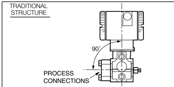
Figure 4. Vertical Mounting Showing Process Connections at 90 degrees
