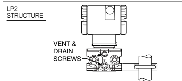
Figure 14. Shown on Foxboro Universal Bracket
