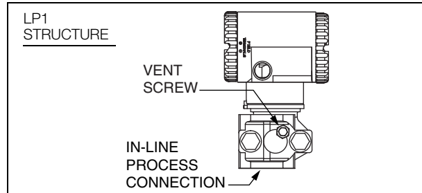
Figure 11. Upright Mounting
