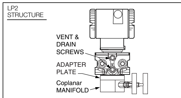
Figure 16. Adapter Mount to Existing Coplanar Manifold
