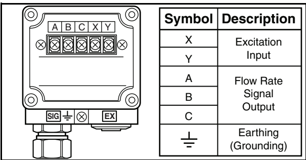
Figure 6. MAG2RS Terminals
