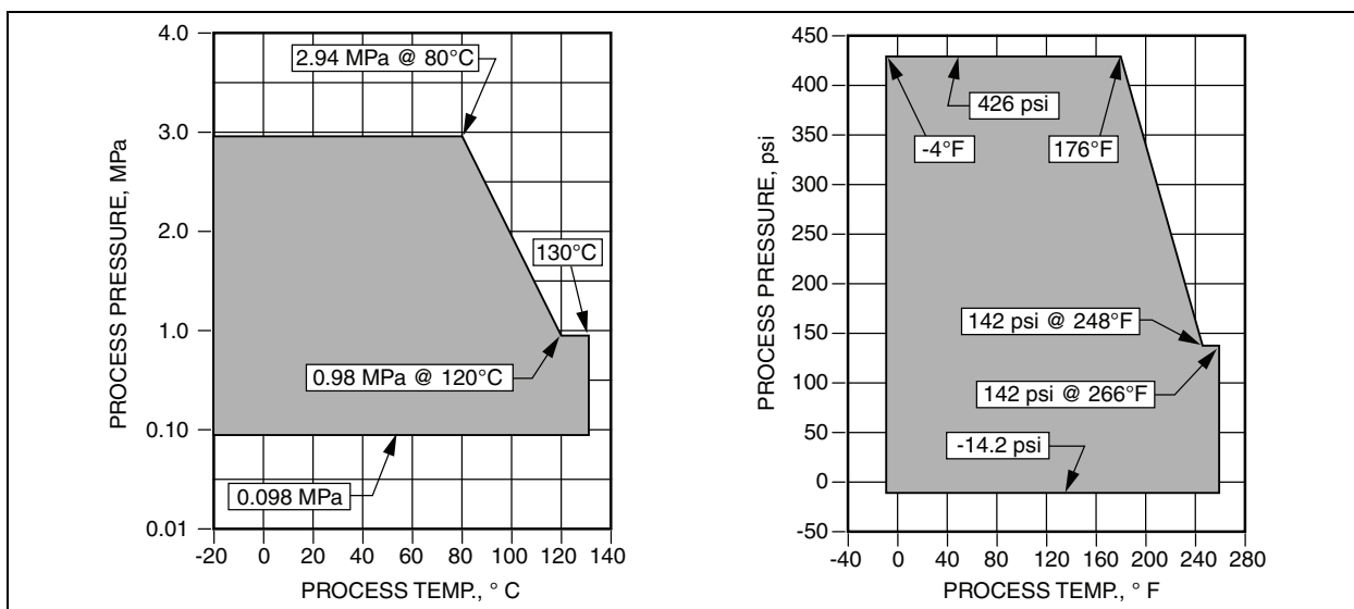
Figure 2. Nominal Line Sizes 15 to 200 mm (1/2 to 8 in) Process Temperature/Process Pressure Ranges
