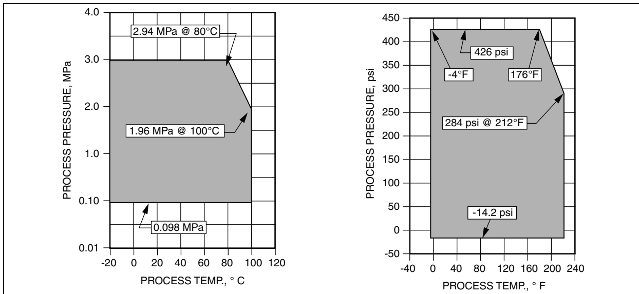
Figure 1. Nominal Line Sizes 2.5 to 10 mm (0.1 to 3/8 in) Process Temperature/Process Pressure Ranges
