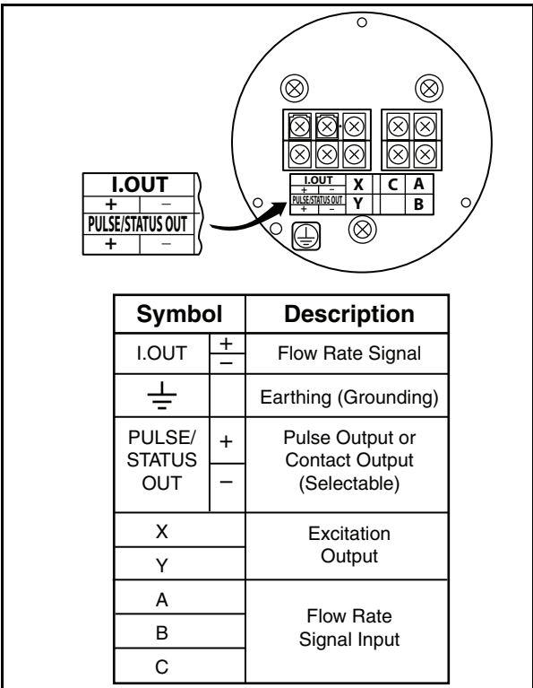
Figure 5. MAG2RT Terminals
