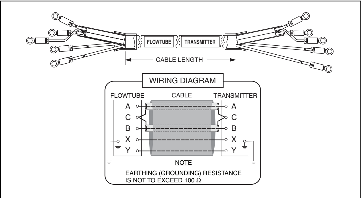
Figure 8. Cable Assembly for Interconnecting the Model MAG2RS Flowtube with the Model MAG2RT Remote Mounted Transmitter
