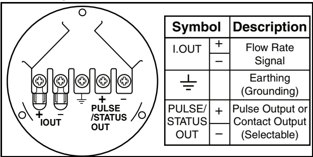
Figure 4. MAG2IC Terminals
